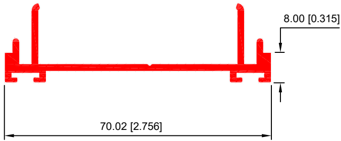
MULLION 40287
