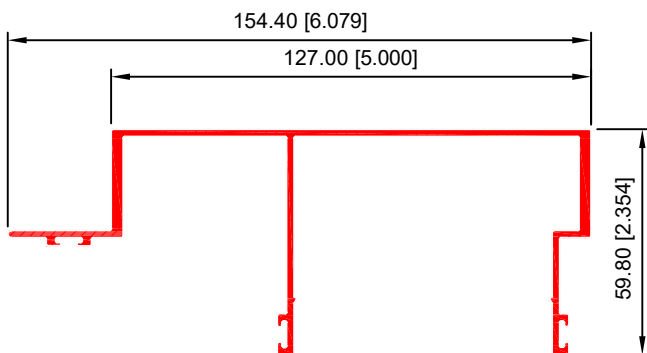
MACHO VERTICAL 40087
