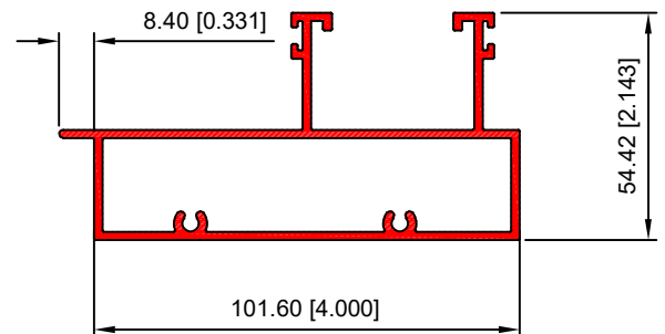
MACHO HORIZONTAL 40548
