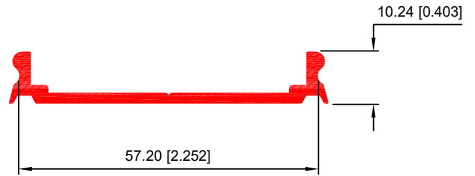
MULLION 2.5'' 40138
