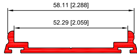
40524-GRAPA 2.4"
