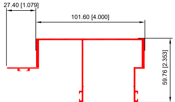
MACHO VERTICAL 40047
