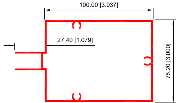
BASICO VERTICAL 40231
