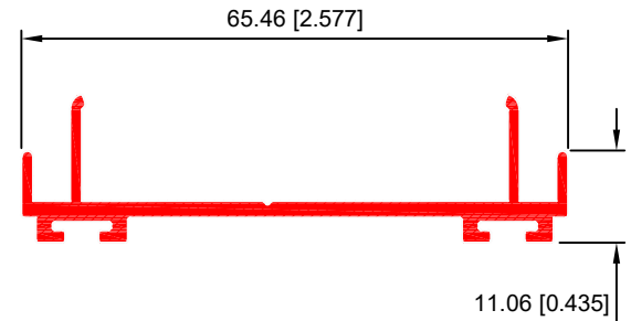
MULLION 2.5'' 40189
