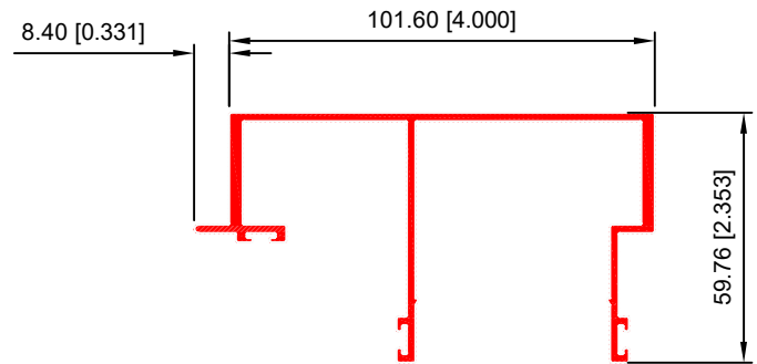
MACHO VERTICAL 40546
