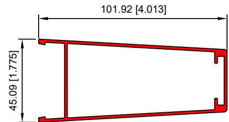
40564-PARTELUZ 4"
