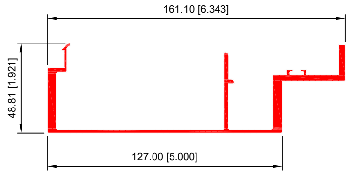
MACHO VERTICAL 5'' 40034
