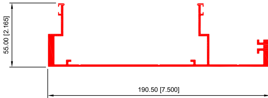
MACHO VERTICAL 40180
